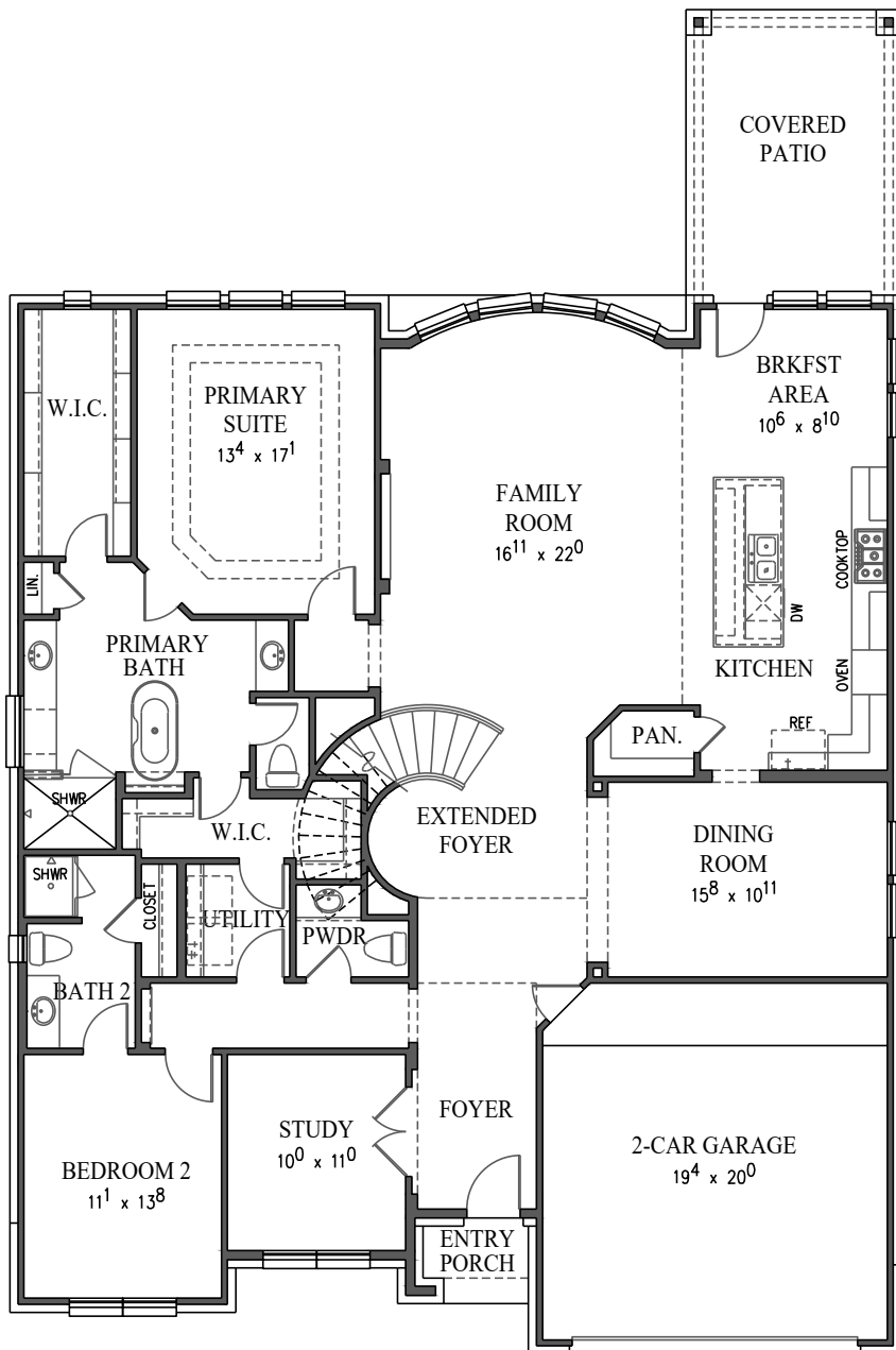
FIRST FLOOR
